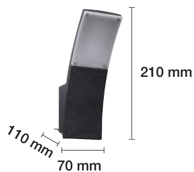
APLIQUE LED 6W PARED IP54 PF>0,9
